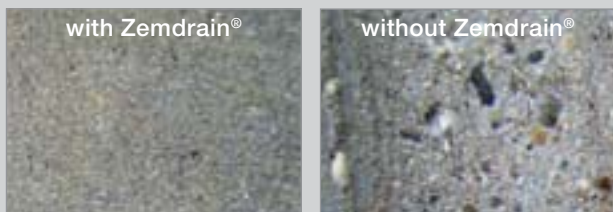
Picture 1: Visual difference between concrete walls produced with Zemdrain® and without Zemdrain® at the walls of the wastewater treatment plant Offenburg after 10 years of operation.
