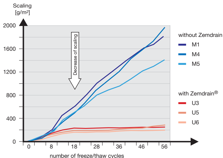
Result of scaling in g/m 2 after 56 frost/thaw cycles (refer to analysis of FEhS 2008/310)
